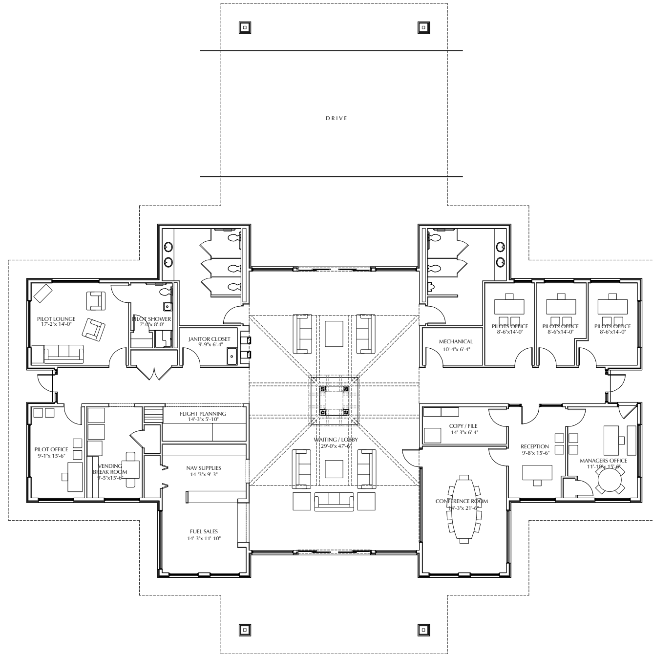
FLOOR PLAN SCALE 1/8" = 1'-0" 4974 SQUARE FEET
